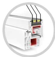
T-Perfekt 6 chambers frame depth 82 mm
