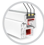
T-Perfekt 6 chambers depth of frame: 82 mm
