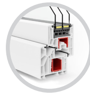
T-Energy 6 chambers depth of frame: 88 mm
